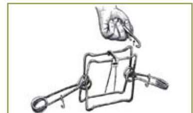
Figure MN4b. Using safety gripper
